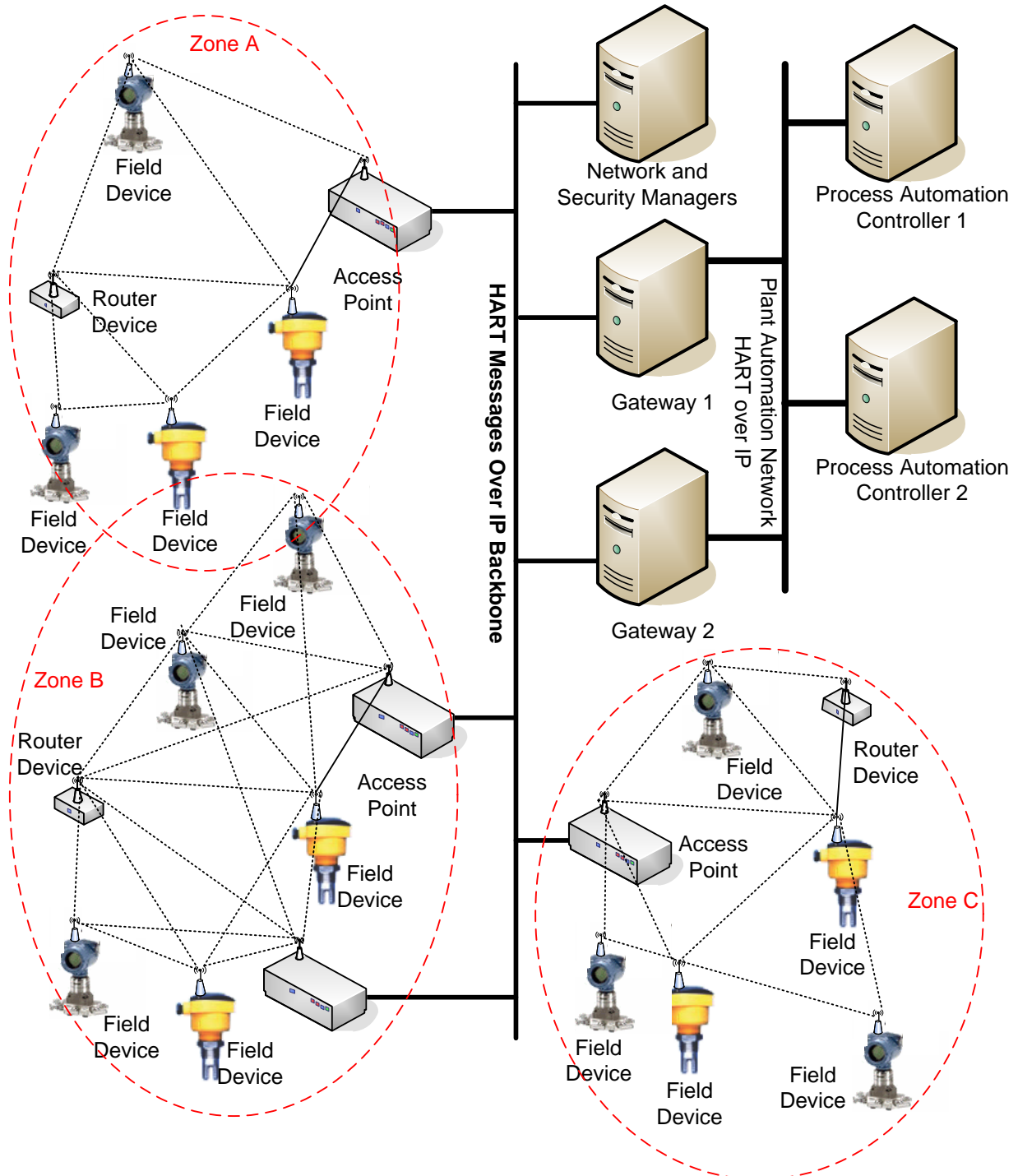
Figure 2 – Utilizing a single backbone to connect multiple access points
