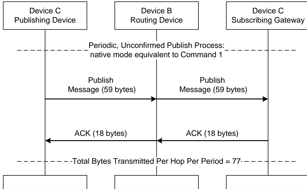
Figure 7 – ISA100.11a Packets
