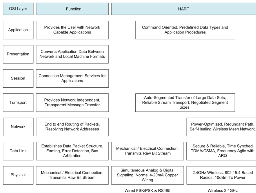
Figure 3 – WirelessHART Layers
